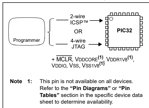
FIGURE 4-1: PROGRAMMING INTERFACES
